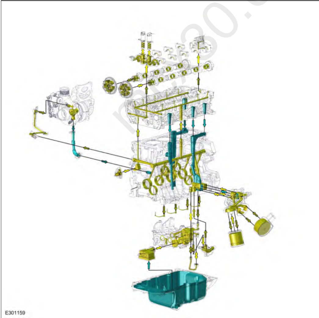
Oil Flow Diagram
